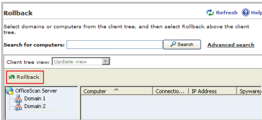
FIGURE 2-13. Rollback screen
